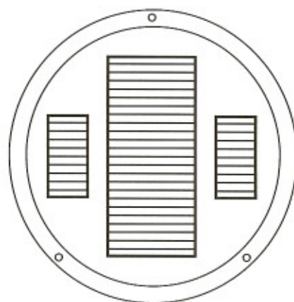
Mounting: 3 Holes - 120° on Diameter of 6"
